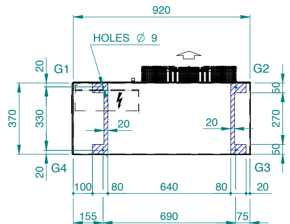
FOOTPRINT
