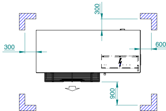
CLEARANCES
