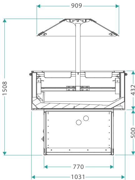
SIDE SECTION VIEW
